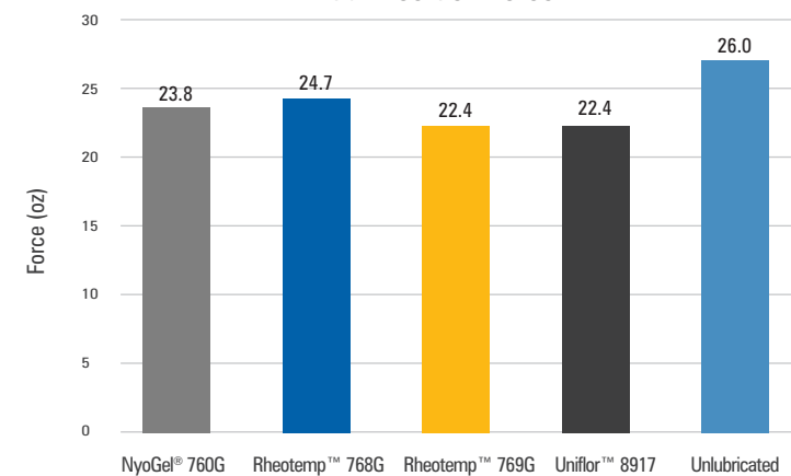
Initial Insertion Force
