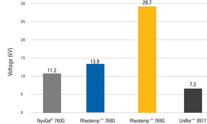
Voltage Breakdown Point
